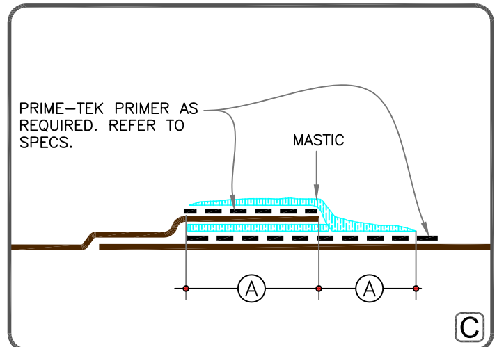
REPAIR STEP 2
