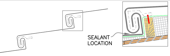
F BERMUDA TYPE ROOF (HORIZONTAL SEAMS)
