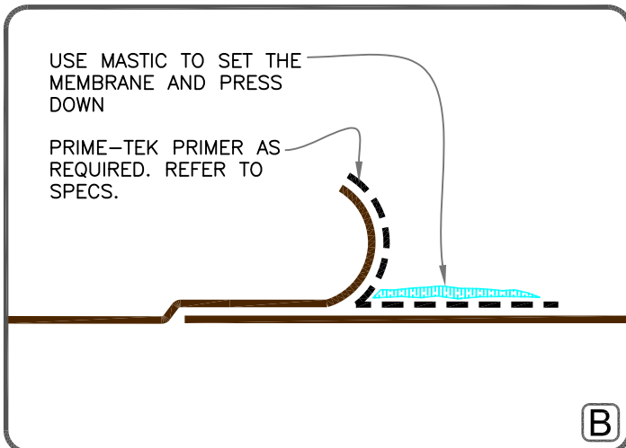
REPAIR STEP 1
